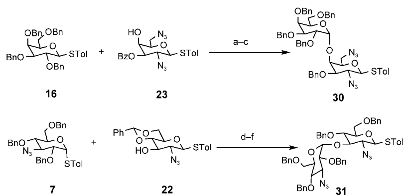
Scheme 2. Representative synthesis of disaccharide building blocks. a) NIS, TfOH, \text{CH}_2\text{Cl}_2 , mol. sieves (4 Å), -45^\circ\text{C} ; b) NaOMe/MeOH; c) NaH, BnBr, TBAI, DMF, 54% (three steps); d) NIS, TfOH, \text{CH}_2\text{Cl}_2 , mol. sieves (4 Å), -45^\circ\text{C} ; e) AcOH, \text{H}_2\text{O} , 80^\circ\text{C} ; f) NaH, BnBr, TBAI, DMF, 41% (three steps). NIS = N-iodosuccinimide.
