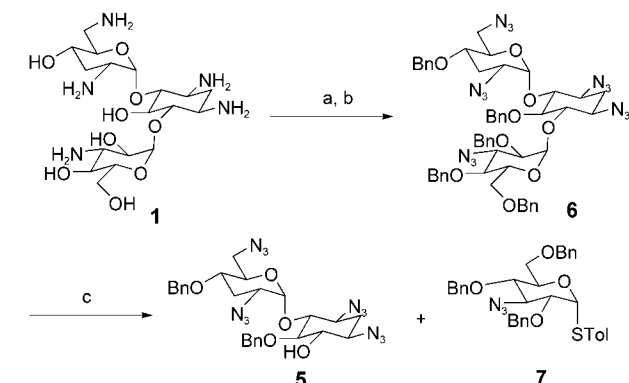
Scheme 1. Synthesis of the protected nebramine core: a) \text{TfN}_3 , \text{ZnCl}_2 (cat.), \text{NEt}_3 , \text{CH}_2\text{Cl}_2 , \text{H}_2\text{O} , \text{MeOH} ; b) \text{NaH} , \text{BnBr} , \text{TBAI} , \text{DMF} , 82% (two steps); c) p -TolSH, \text{BF}_3 \cdot \text{Et}_2\text{O} , \text{CH}_2\text{Cl}_2 , 5 43%, 7 47%. Tf = triflate ( \text{CF}_3\text{SO}_2 ), Bn = benzyl, TBAI = tetra- n -butylammonium iodide, DMF = N,N -dimethylformamide.
