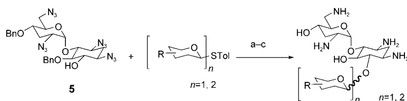
Scheme 3. Synthesis of tobramycin analogues. a) BSP, \text{TiF}_4 , \text{CH}_2\text{Cl}_2 , mol. sieves (4 Å), -45^\circ\text{C} , 32–78%; b) Raney Ni, \text{N}_2\text{H}_4 , EtOH, dioxane; c) HCl (0.1 N), \text{H}_2 , \text{Pd}(\text{OH})_2 (20%), MeOH/ \text{H}_2\text{O} , 19–65% (two steps). BSP = benzenesulfinylpiperidine.
